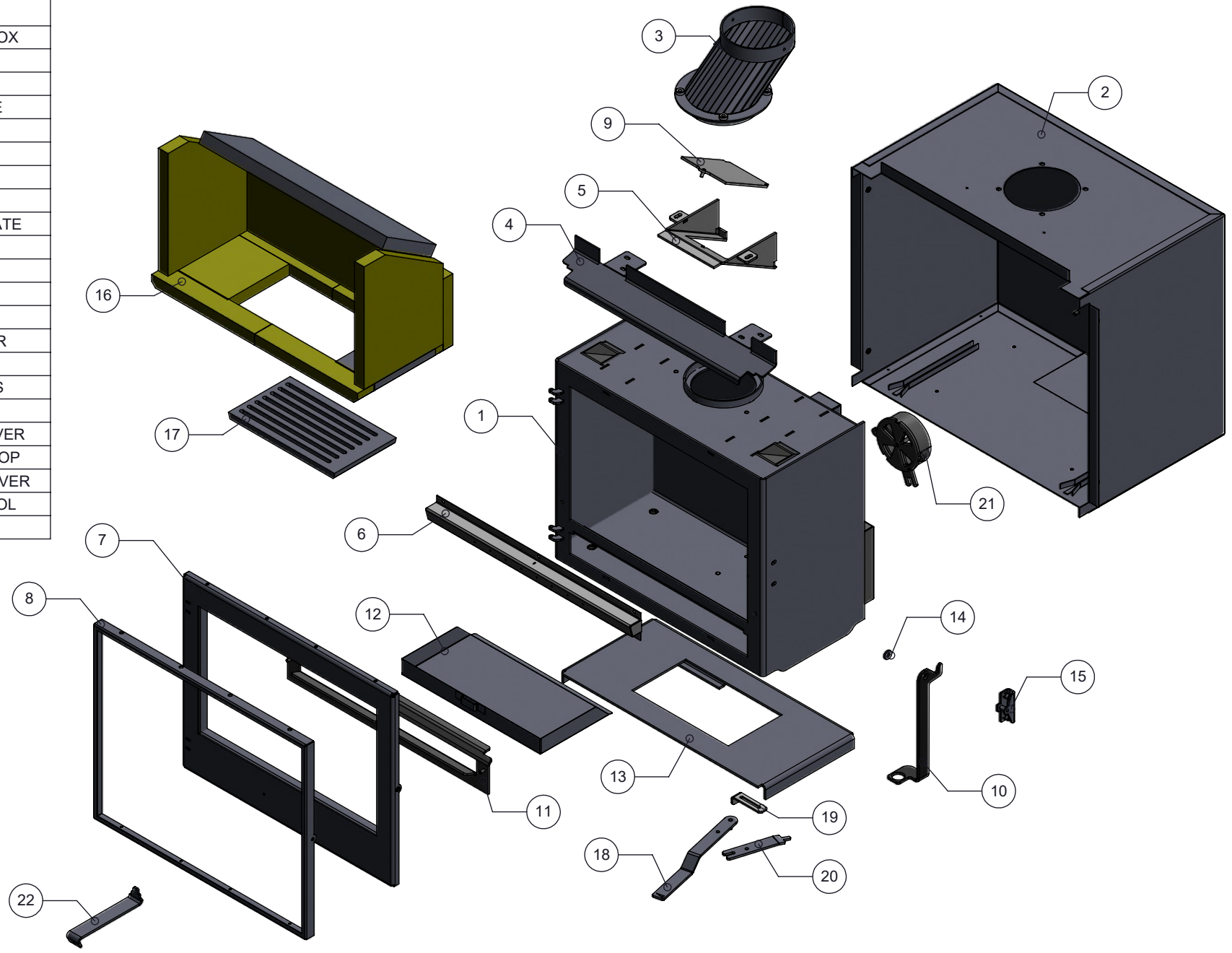
SERENITY 45 INSET EXPLODED VIEW
