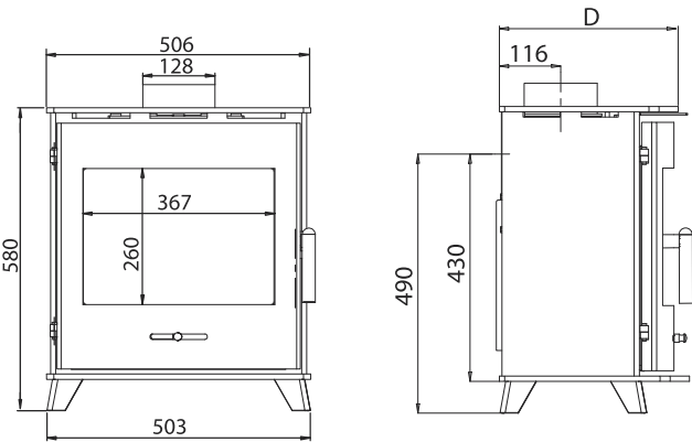
40FS D = 338mm 50FS D = 377mm All Measurements in mm
