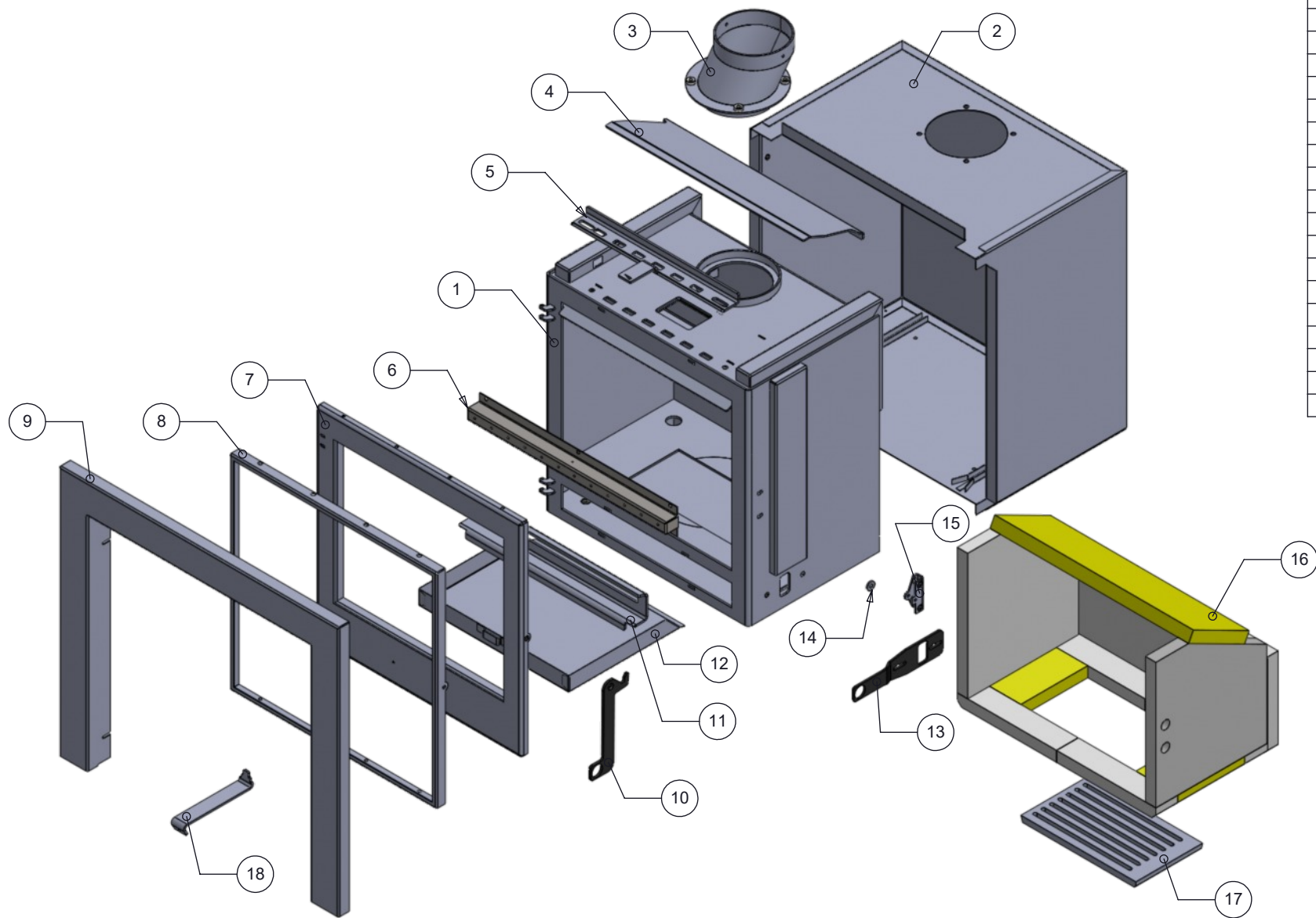
SERENITY 50 INSET EXPLODED VIEW
